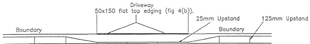
PLAN OF VEHICULAR CROSSOVER
