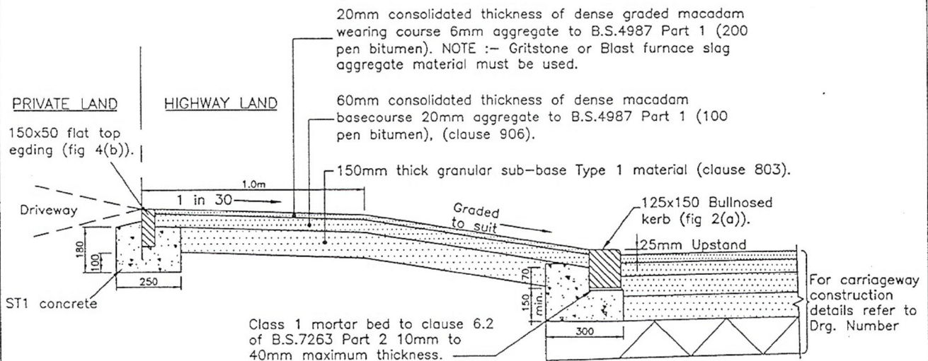
CONSTRUCTION DETAILS
